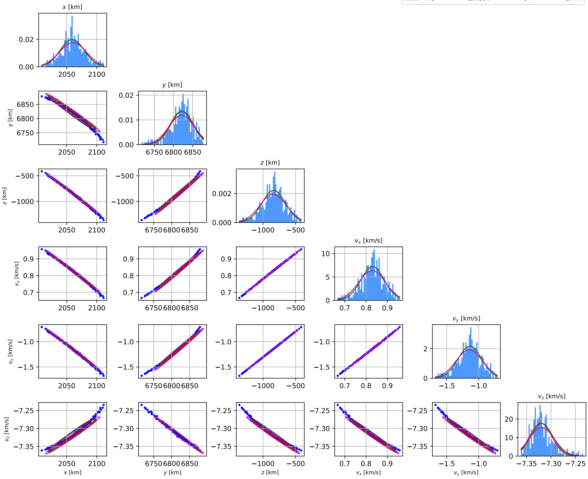
Corner Plot - Time Index 3
