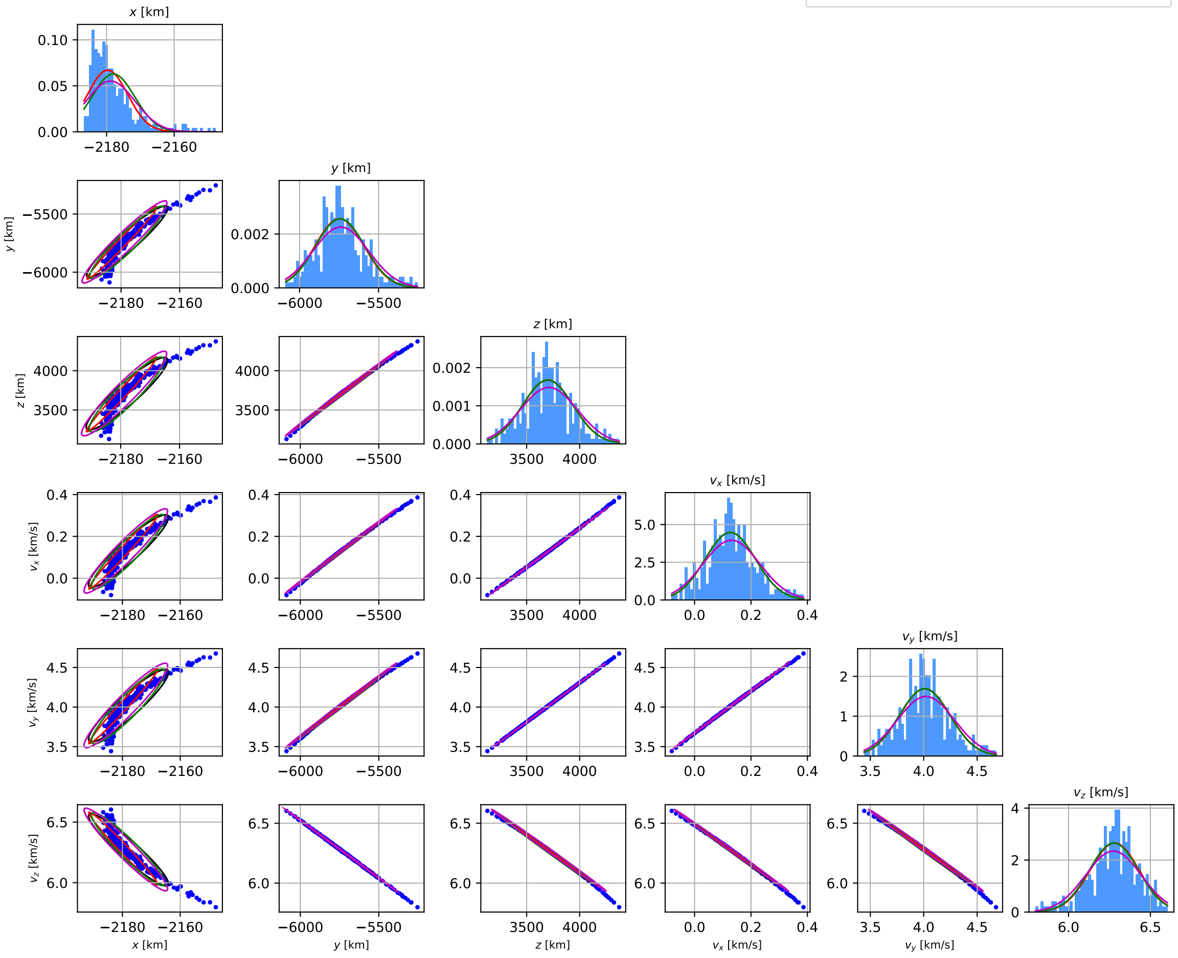
Corner Plot - Time Index 4
