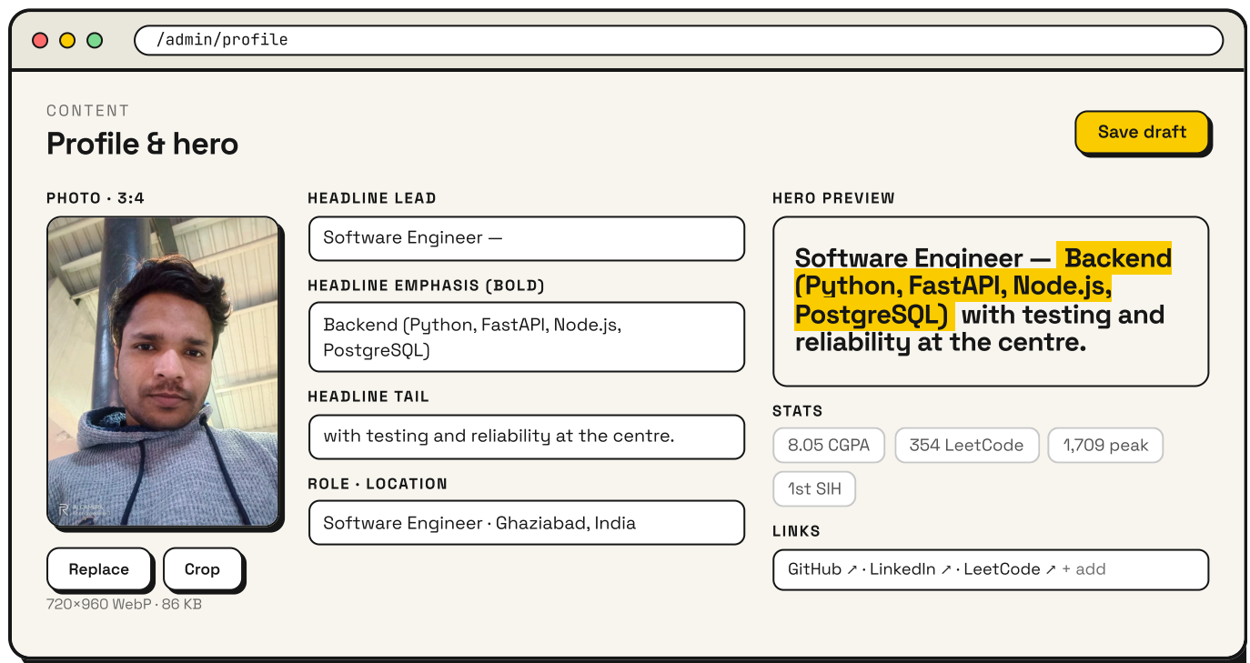
Figure 5: Profile and photo. Uploads are cropped in the browser (canvas) and saved as WebP, so no image library is needed.
