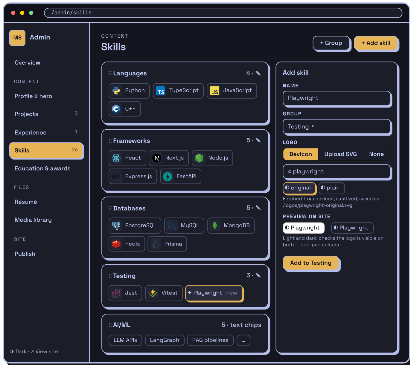
Figure 3: Skills manager in dark mode (Tokyo Night palette from the site). Groups and chips reorder by dragging.
