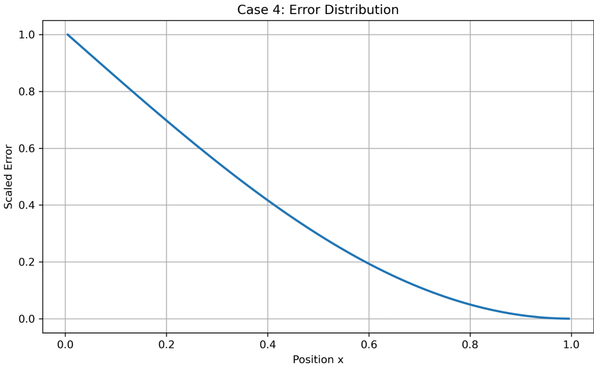
Figure 7. Error distribution between numerical and analytical solutions.
