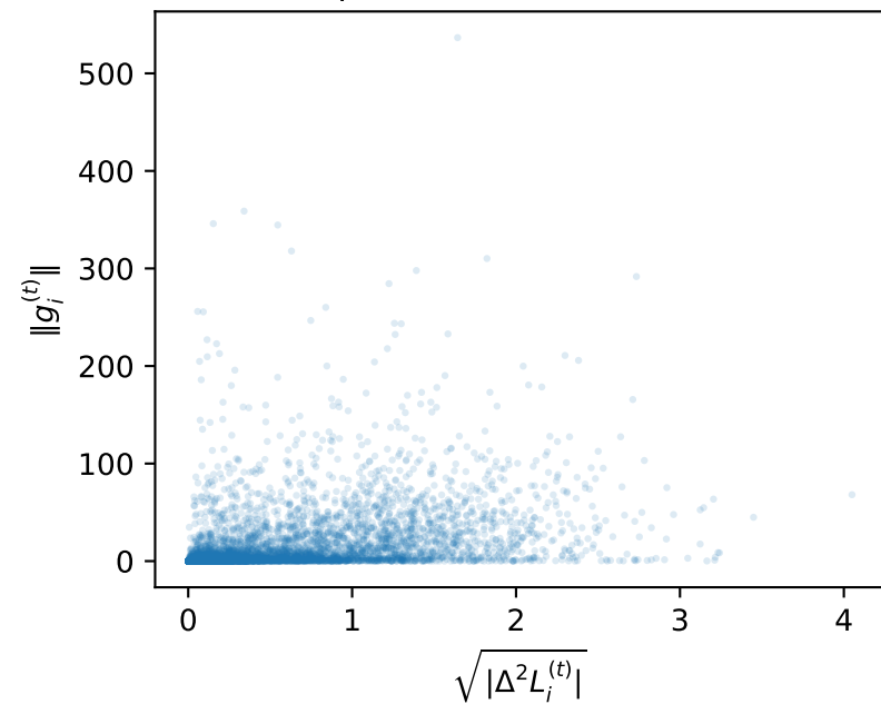
exponential (corr=0.492)
