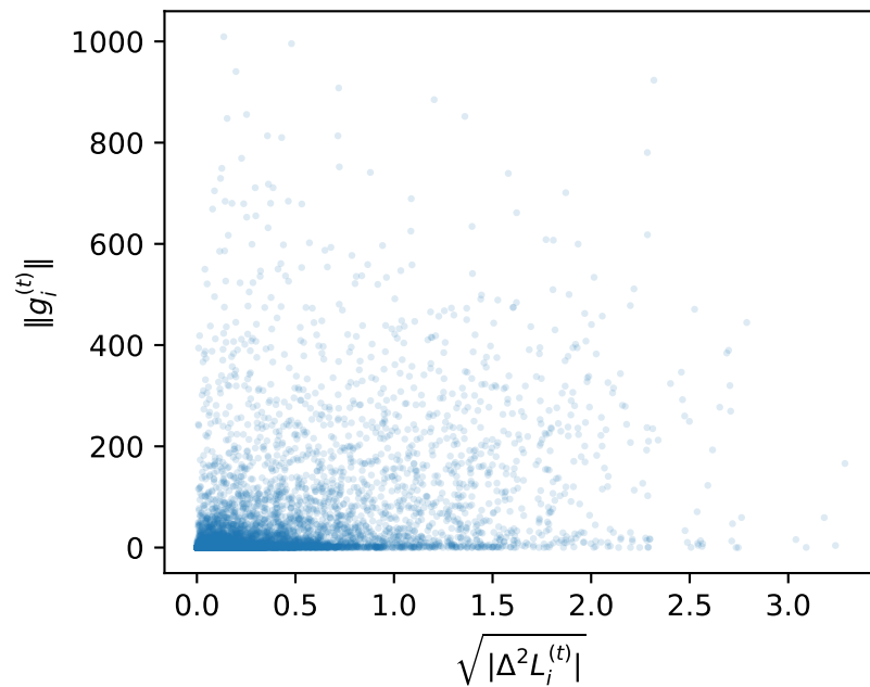
fixed (corr=0.473)
