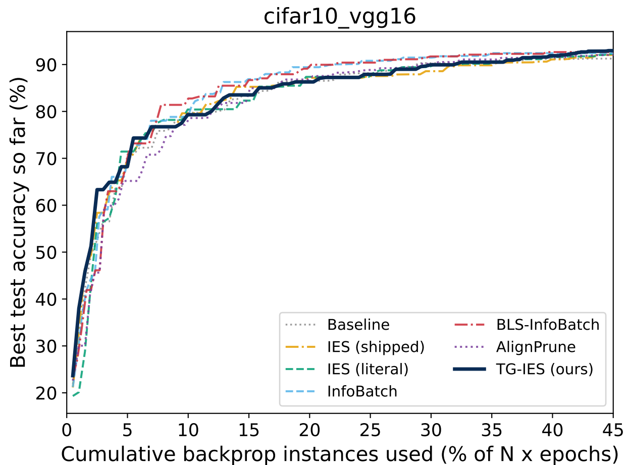
Accuracy vs. compute budget (0-45% shown; all curves are flat beyond this), all cells with new-baseline data
