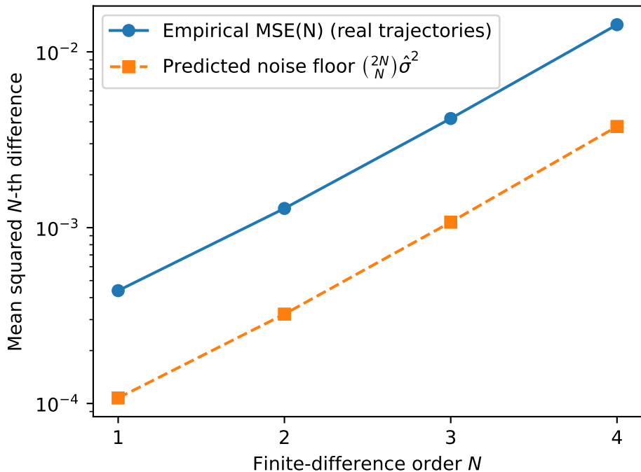
Order-of-difference MSE on real ResNet-18/CIFAR-10 trajectories
