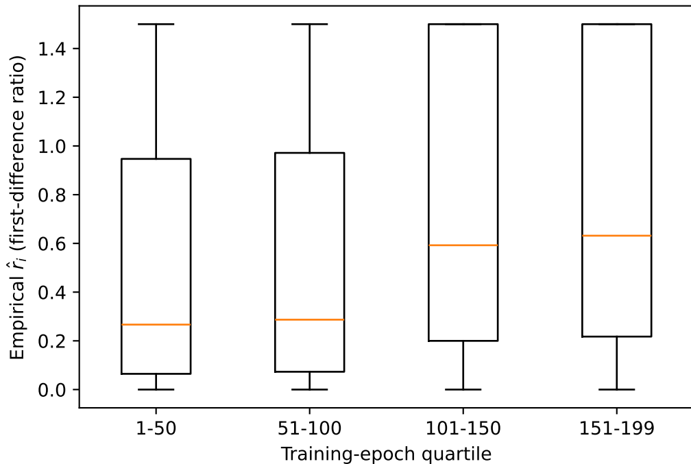
Local decay-rate distribution across training phases
