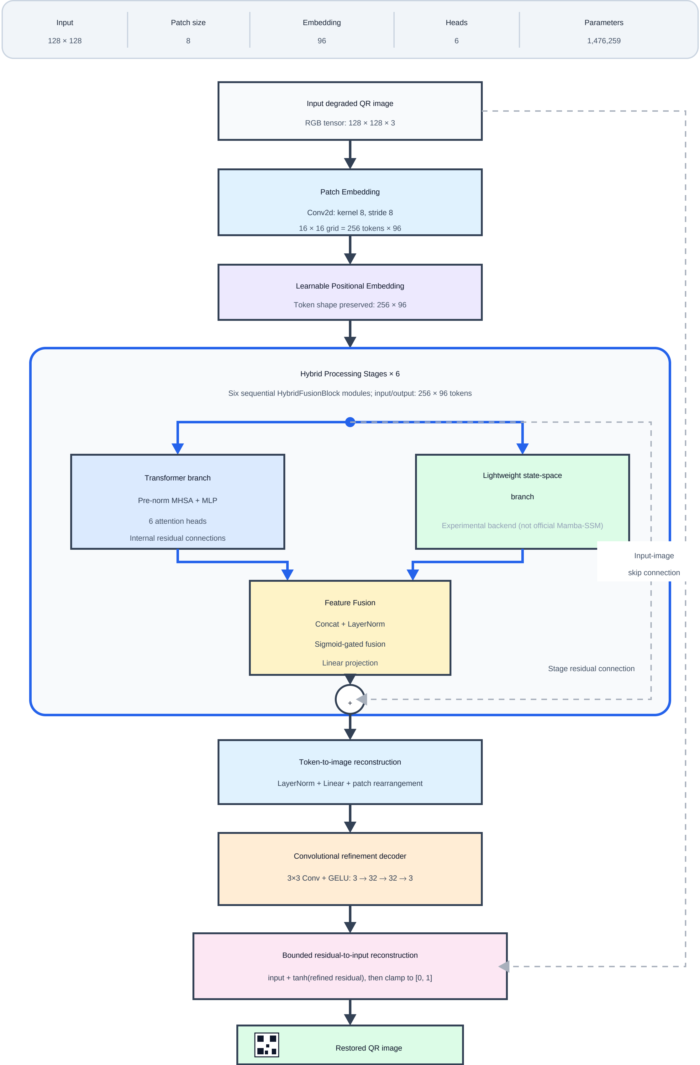
Overall Architecture of the Proposed Mamba-TransQR Framework
