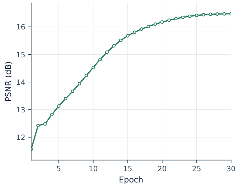
(b) Validation PSNR vs Epoch
