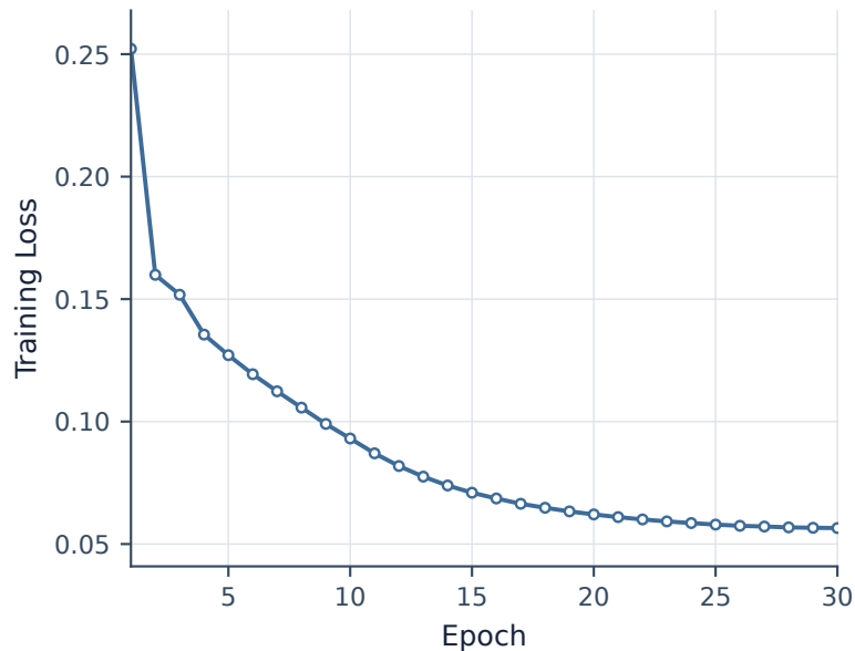
(a) Training Loss vs Epoch
