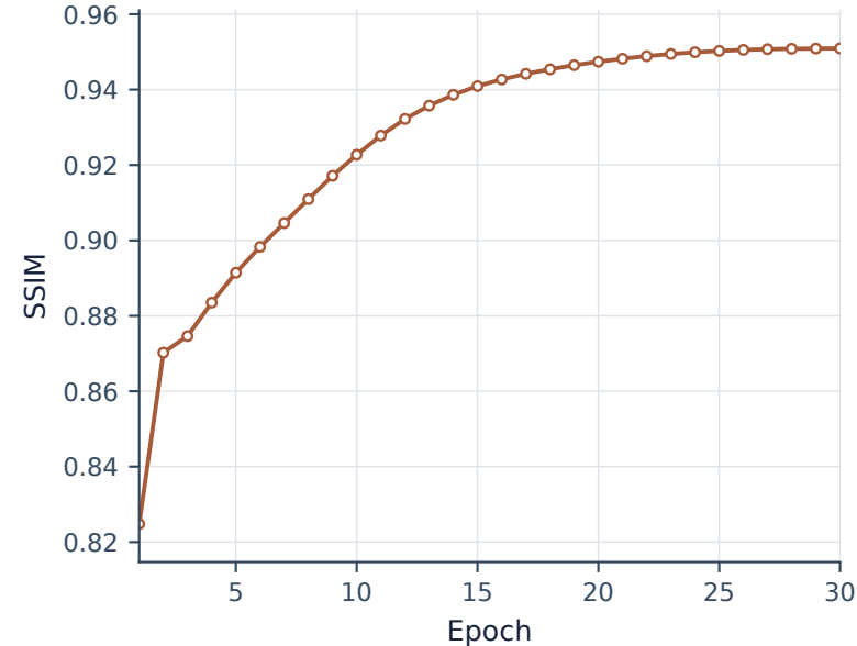
(c) Validation SSIM vs Epoch
