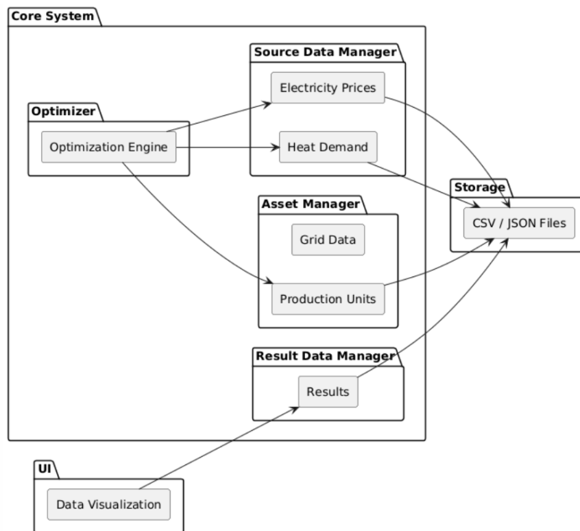
Figure 4.1: Package Diagram
