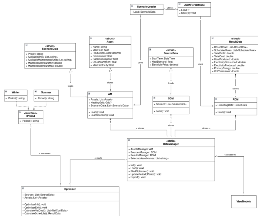
Figure 4.2: Class Diagram
