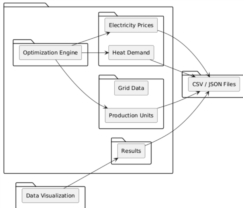
Figure 4.1: Package Diagram
