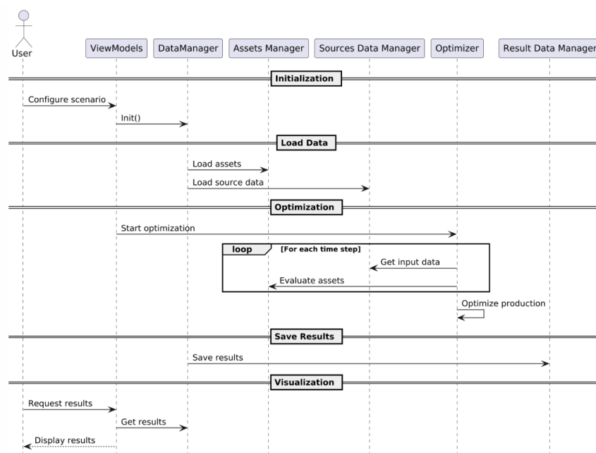
Figure 4.4: Sequence Diagram
