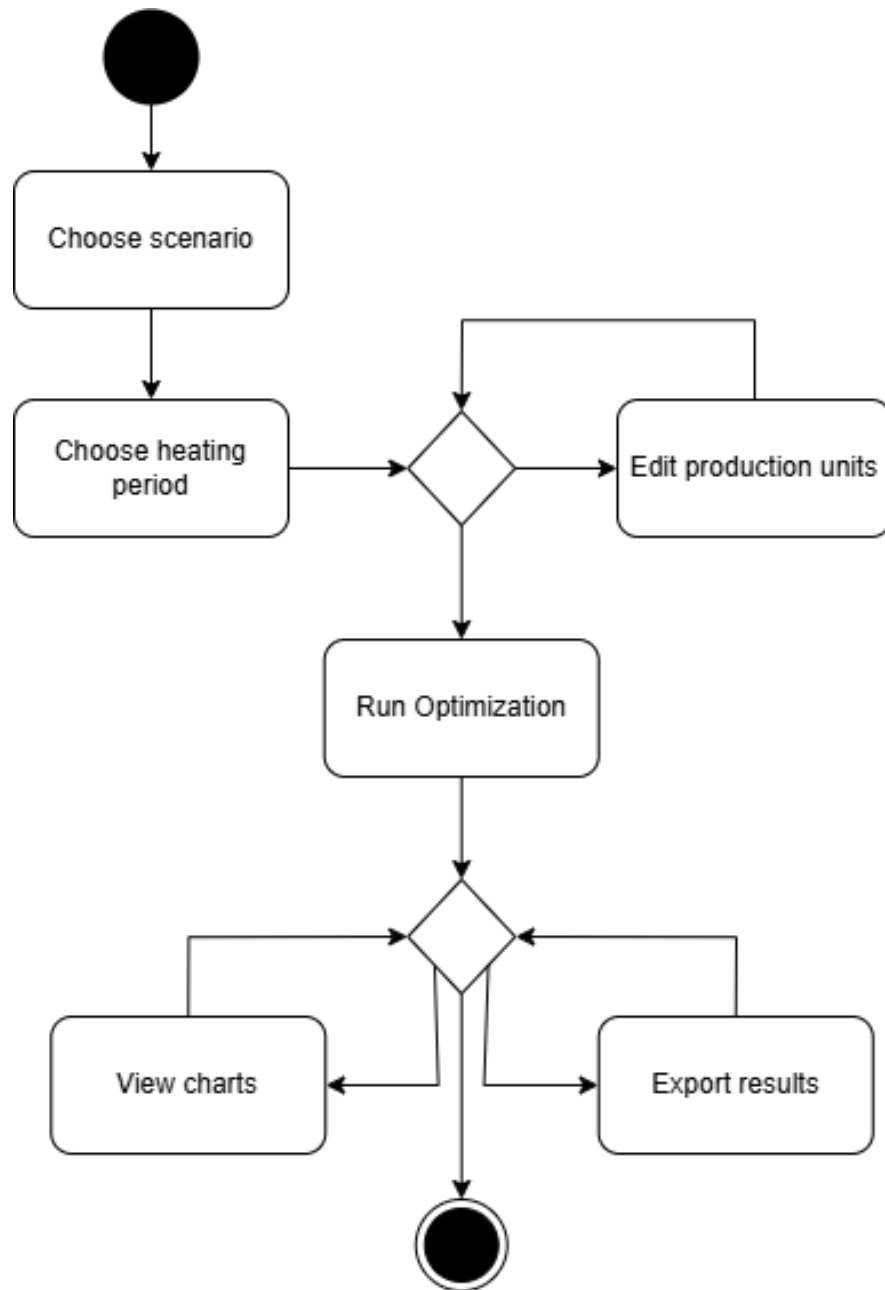
Figure 4.3: Activity Diagram
