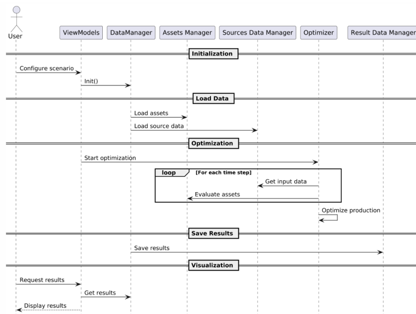
Figure 4.4: Sequence Diagram
