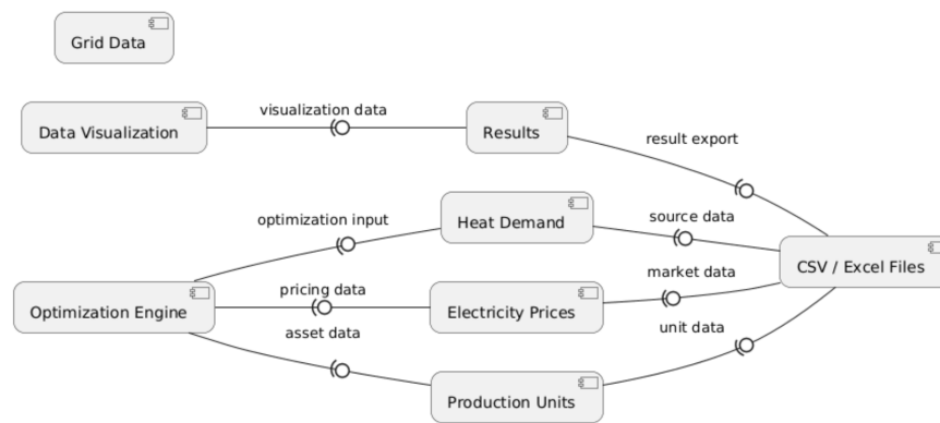
Figure 4.1: Package Diagram
