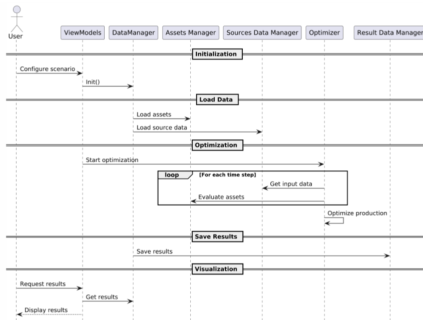
Figure 4.3: Sequence Diagram
