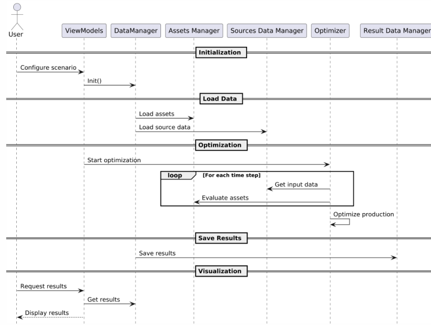
Figure 4.3: Sequence Diagram
