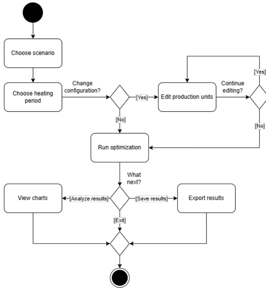
Figure 4.3: Activity Diagram
