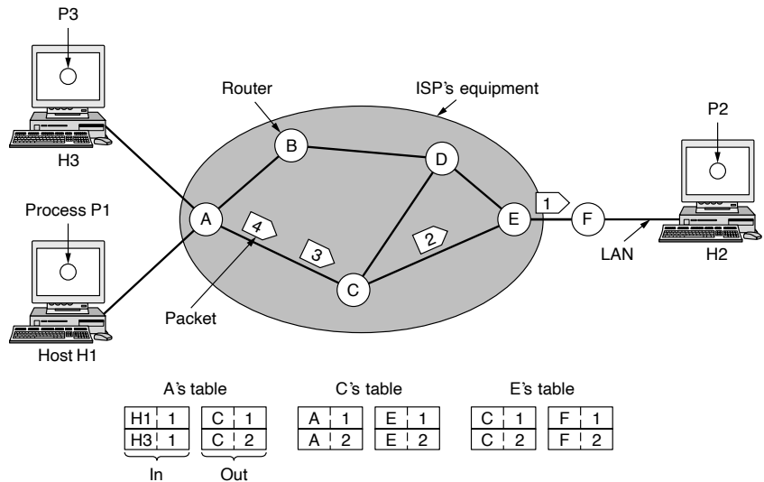
Figure 5-3. Routing within a virtual-circuit network.
