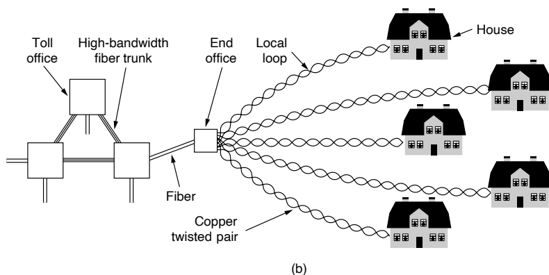
Figure 2-45. (a) Hybrid Fiber-Coax cable network. (b) The fixed phone system.
