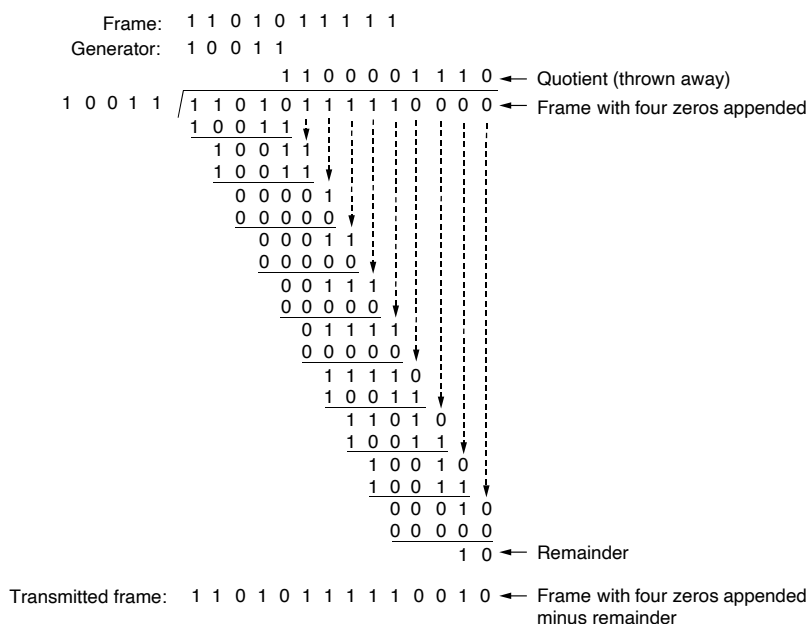
Figure 3-9. Example calculation of the CRC.
