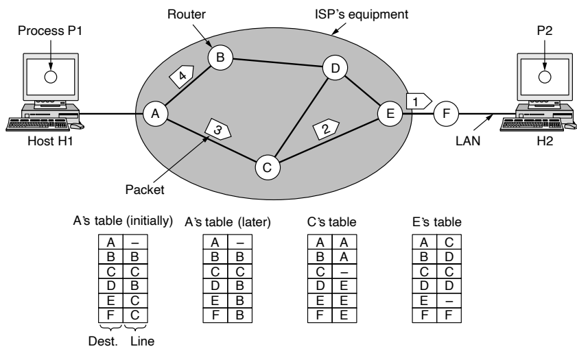
Figure 5-2. Routing within a datagram network.
