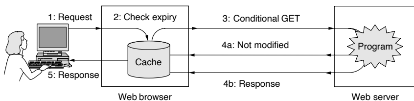
Figure 7-28. HTTP caching.
