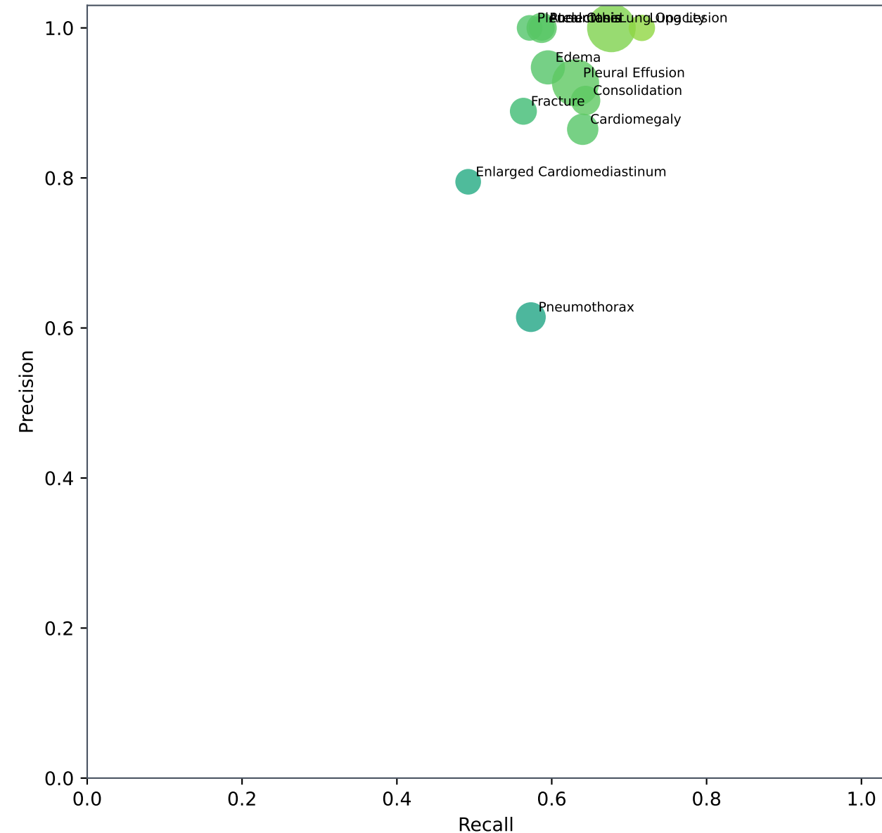
Precision-Recall Trade-off (point size = GT-positive count)
