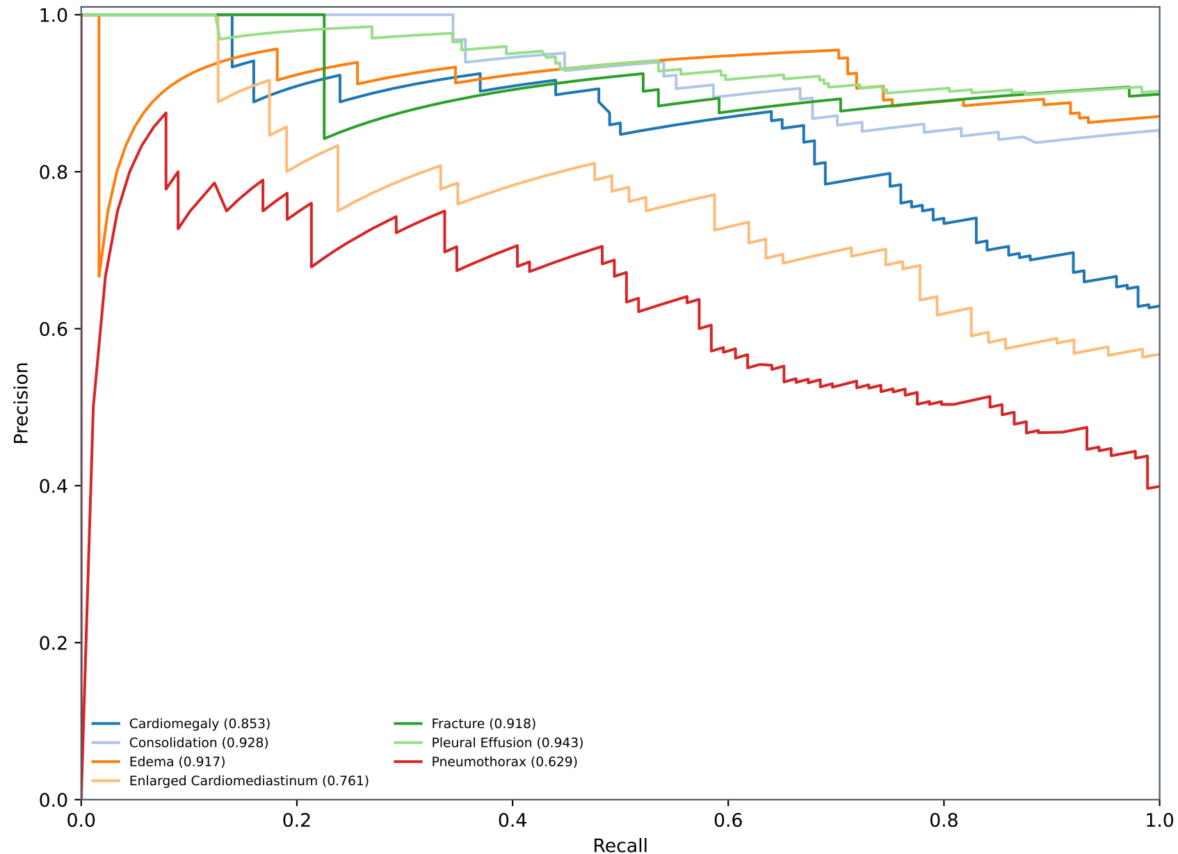
RAD-DINO Precision-Recall Curves — Explicit Present vs Explicit Absent
