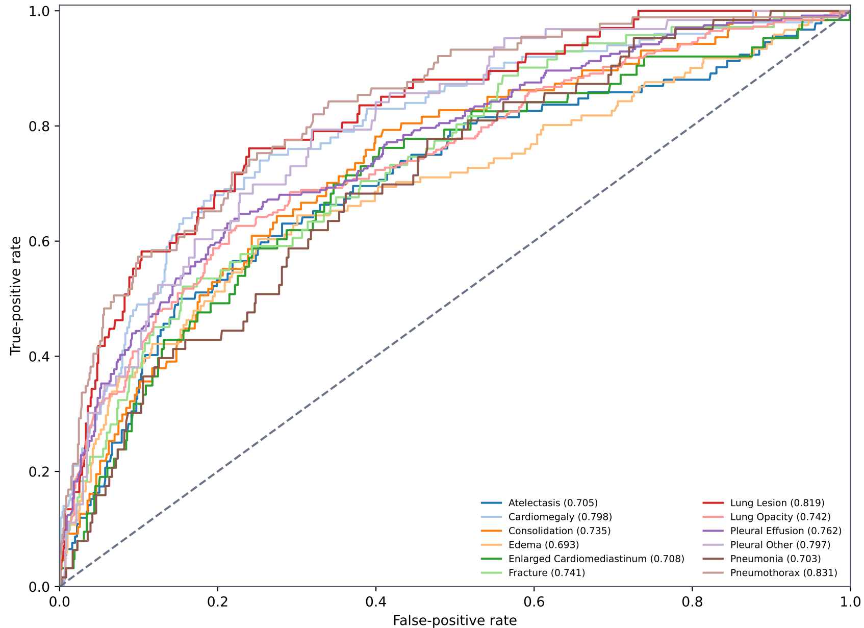
RAD-DINO ROC Curves — Present vs All Other Statuses
