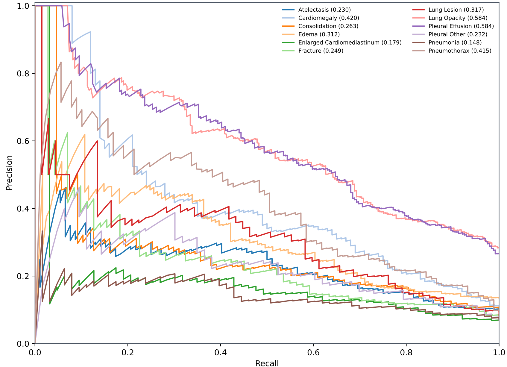
RAD-DINO Precision-Recall Curves — Present vs All Other Statuses
