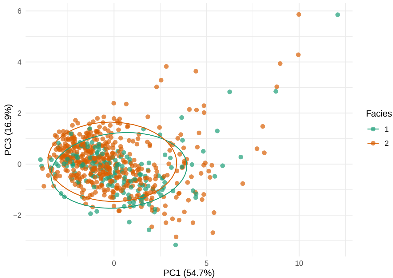
PCA: Redox/Productivity Variables Colored by Facies Class
