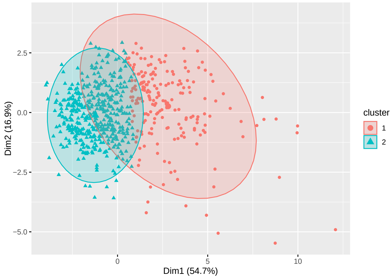
K-means Clustering
