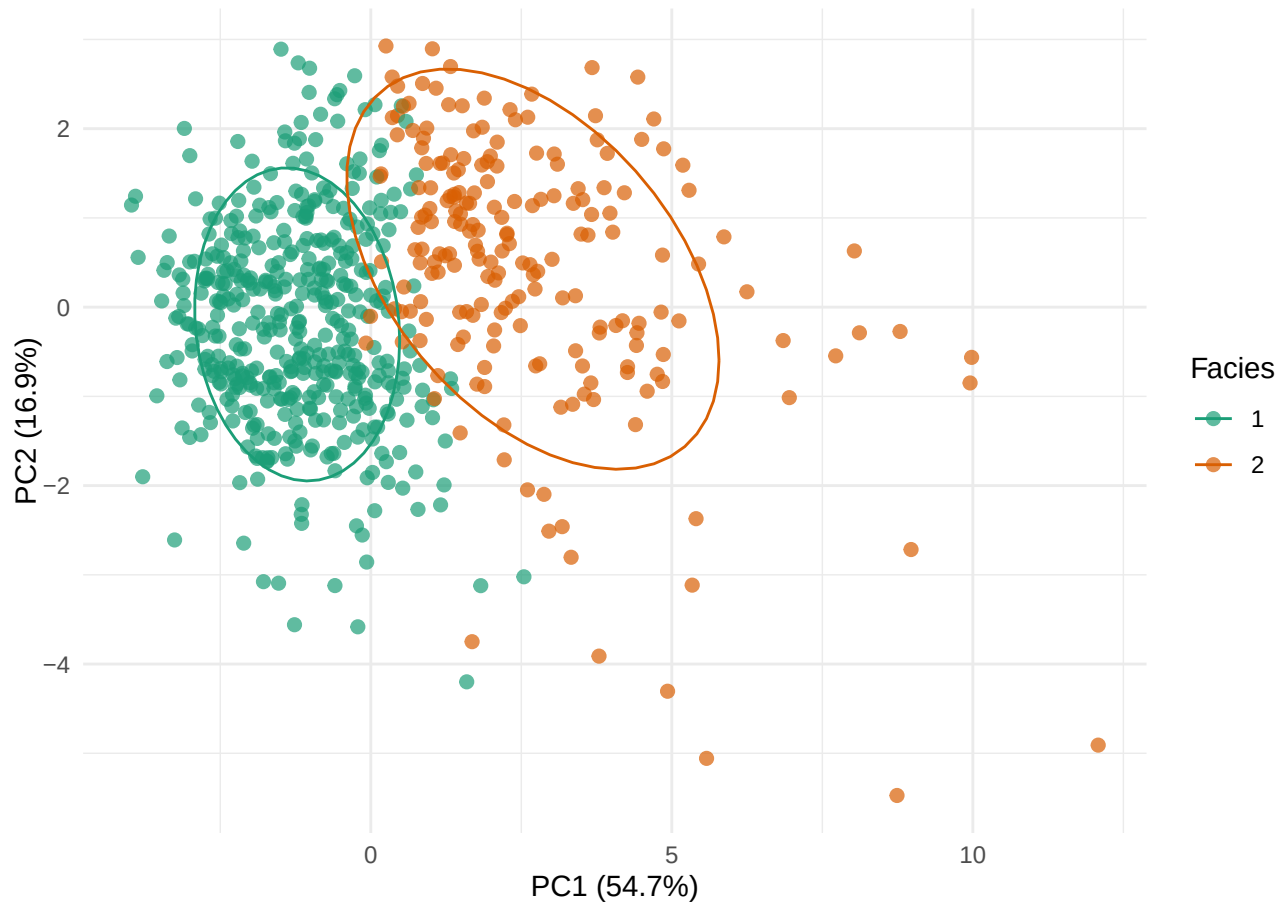
PCA: Redox/Productivity Variables Colored by hclust
