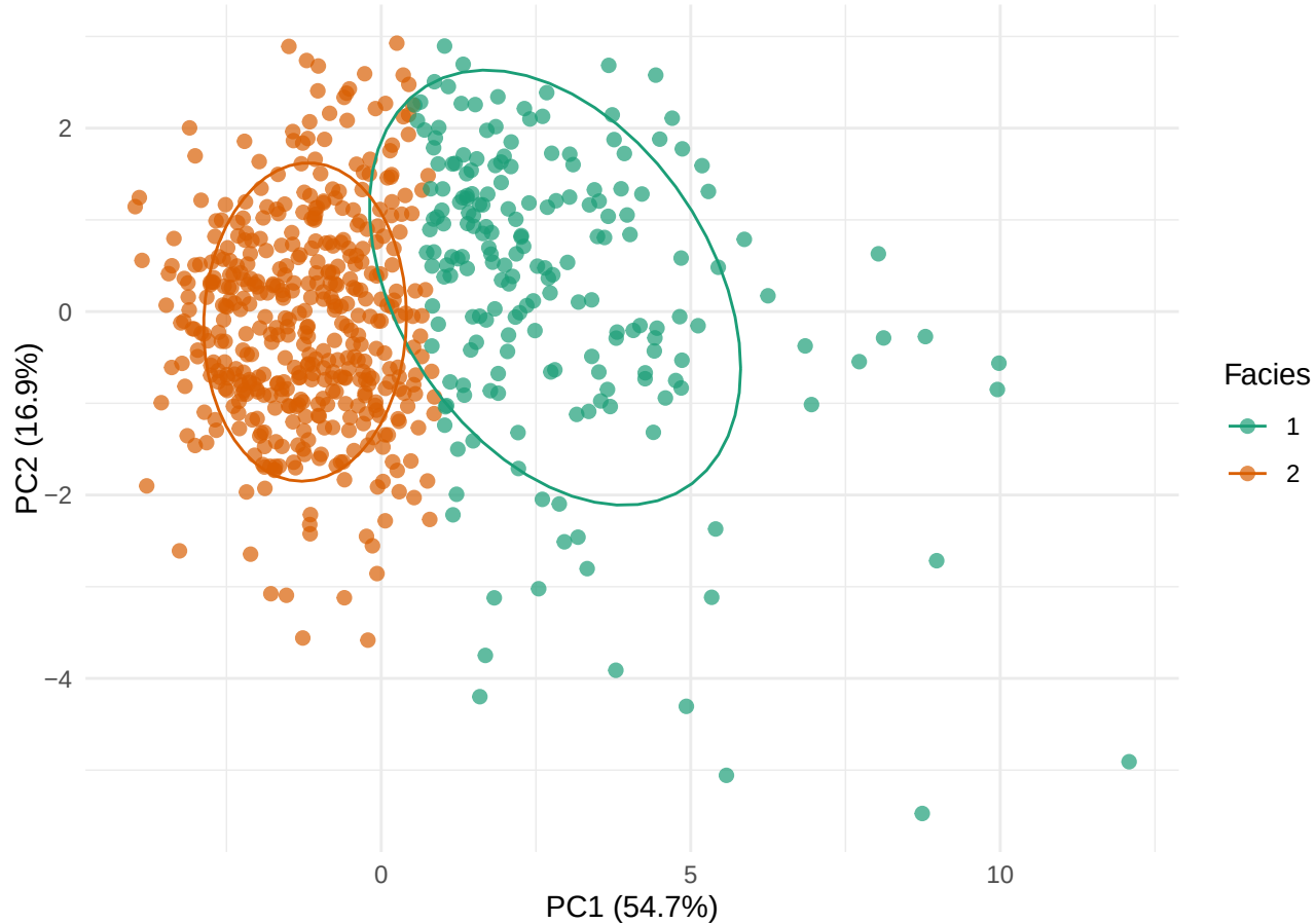
PCA: Redox/Productivity Variables Colored by K-means cluster
