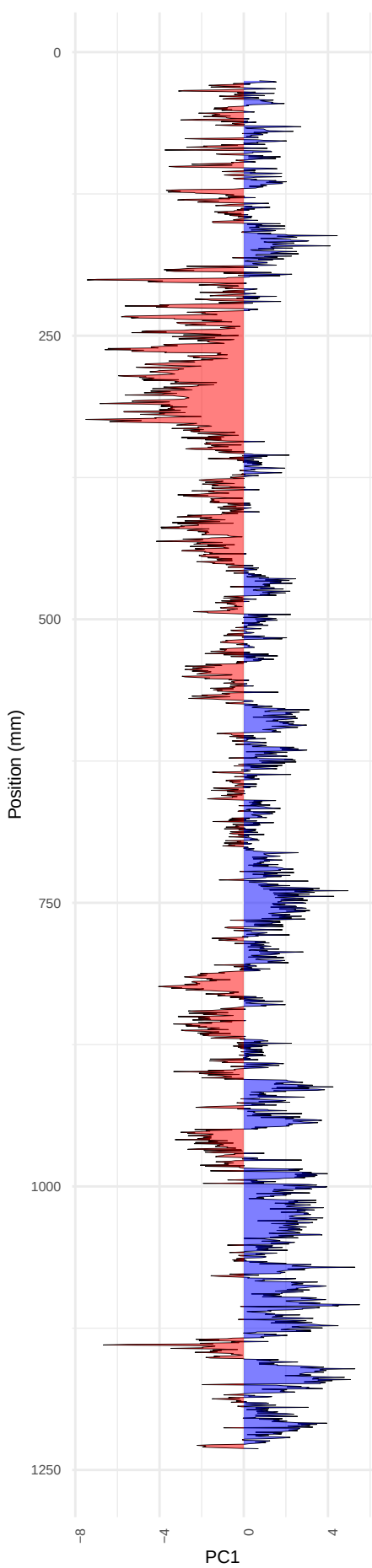
PC1 Variation in clr500_sel_2
