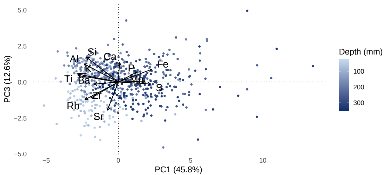
PCA Biplot Colored by Depth – 500µm top 35cm
