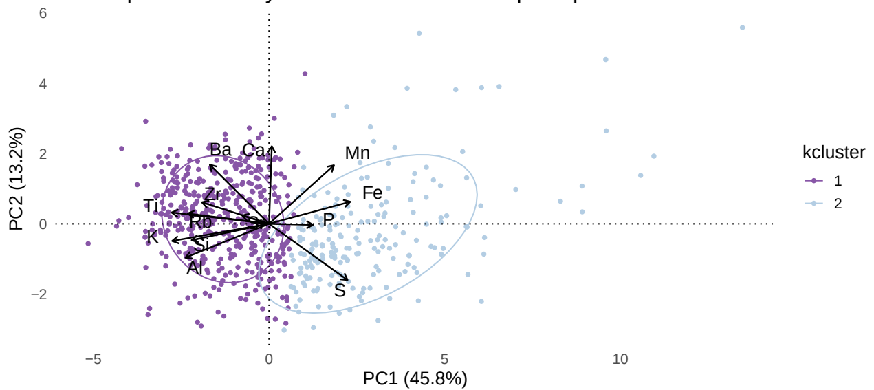
PCA Biplot Colored by K-means Cluster – 500µm top 35cm
