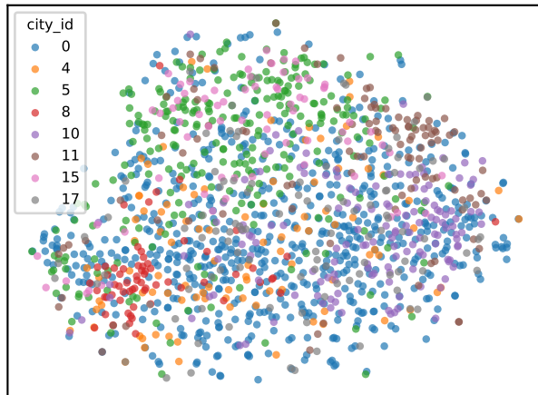
output_decomp_centered color: city_id
