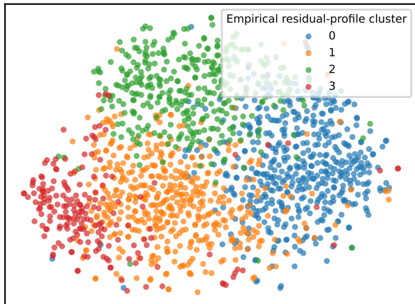
output_decomp_centered color: Empirical residual-profile cluster
