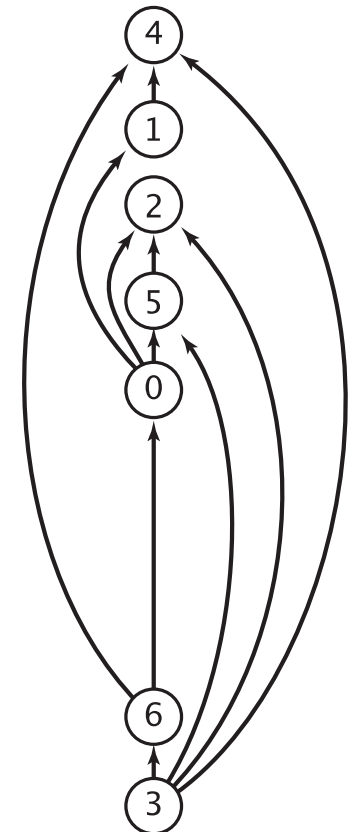
topological order
