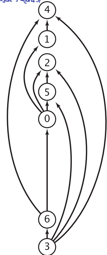
feasible schedule
