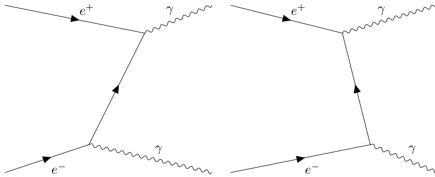
Figure 1: Feynman diagrams for e^+e^- annihilation [1]
