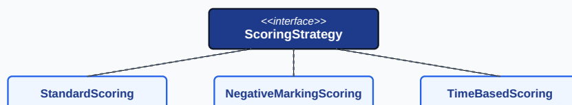
Figure 4.1: Strategy Pattern class structure for modular examination scoring algorithms.
