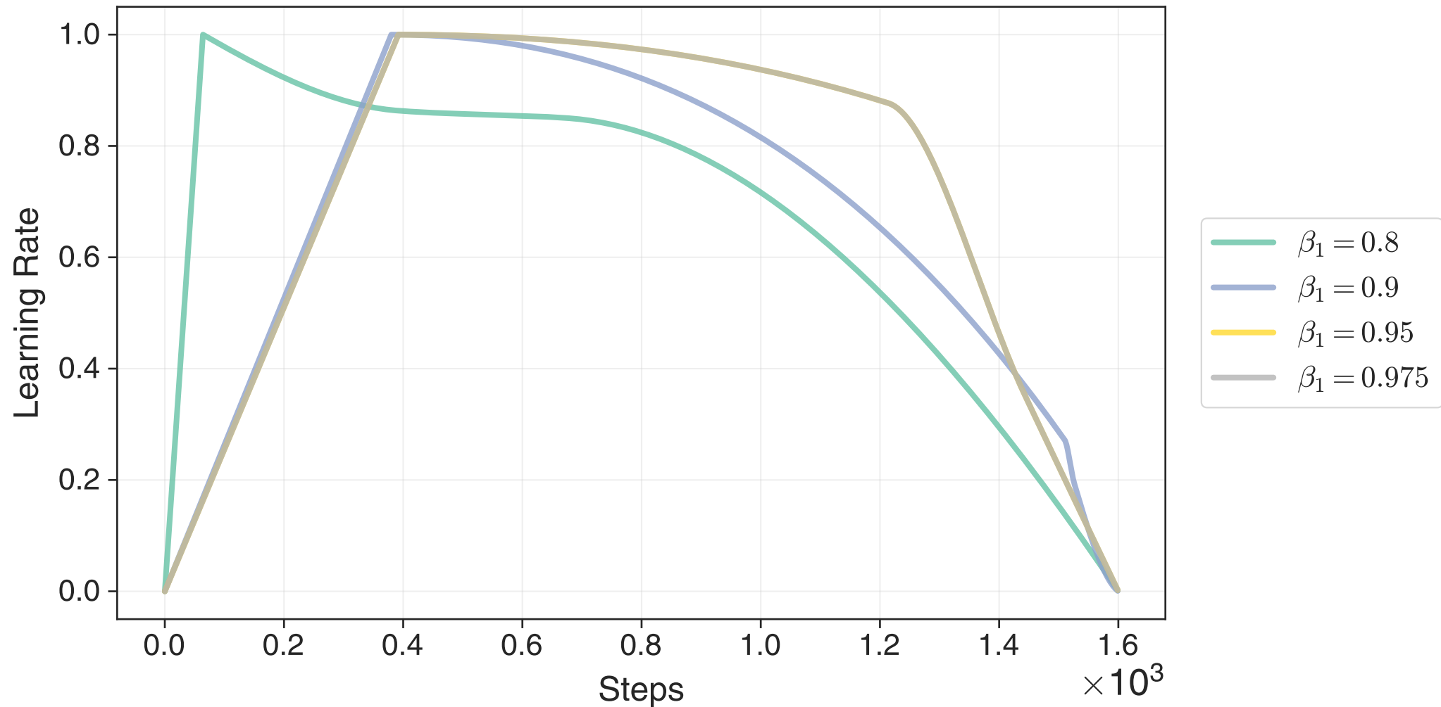
Relative learning rates Wikitext, varying \beta_1 , TPS schedule
