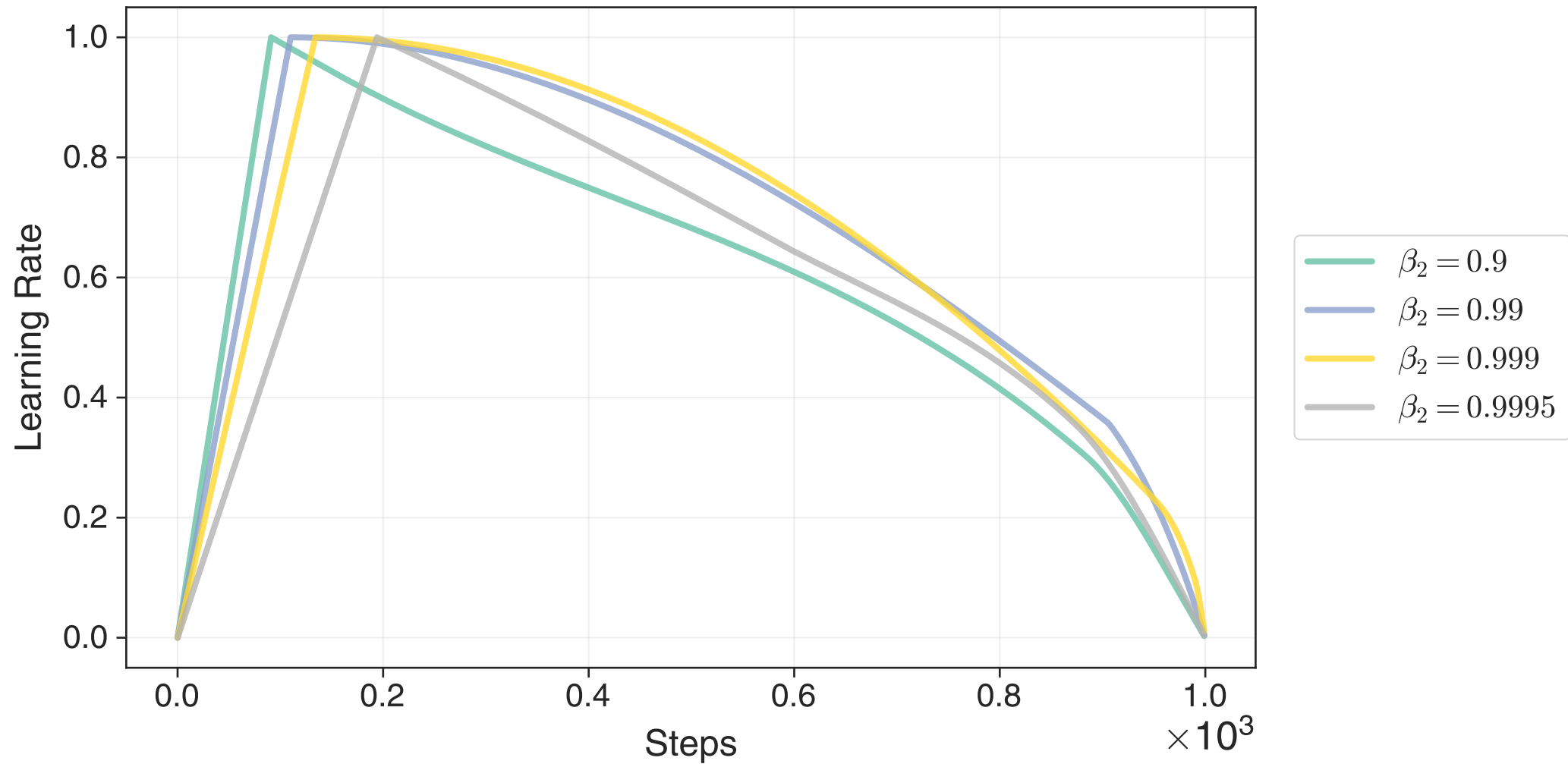
Relative learning rates CIFAR10, varying \beta_2 , TPS schedule
