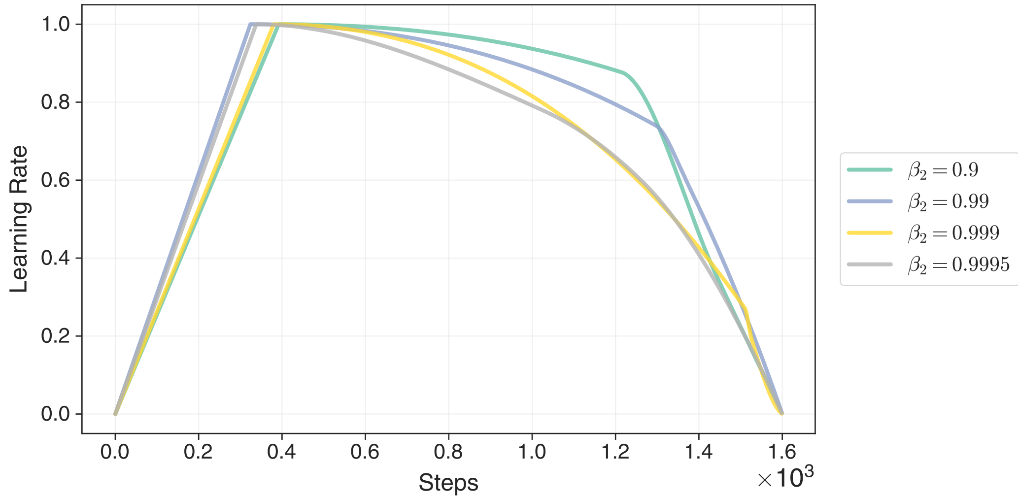
Relative learning rates Wikitext, varying \beta_2 , TPS schedule
