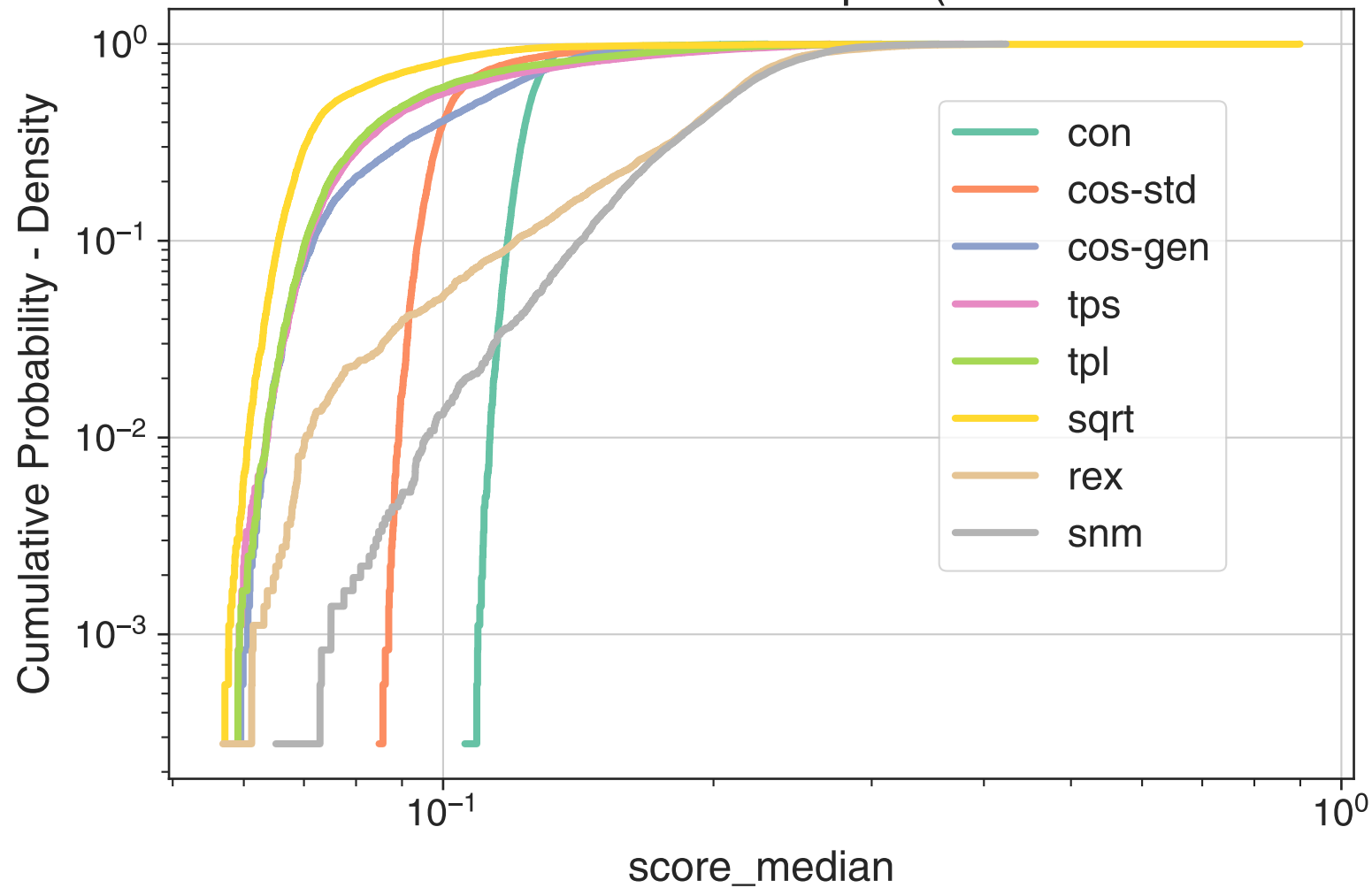
ECDF CIFAR10 search over 3600 shapes (Adam BS256 1000 steps)
