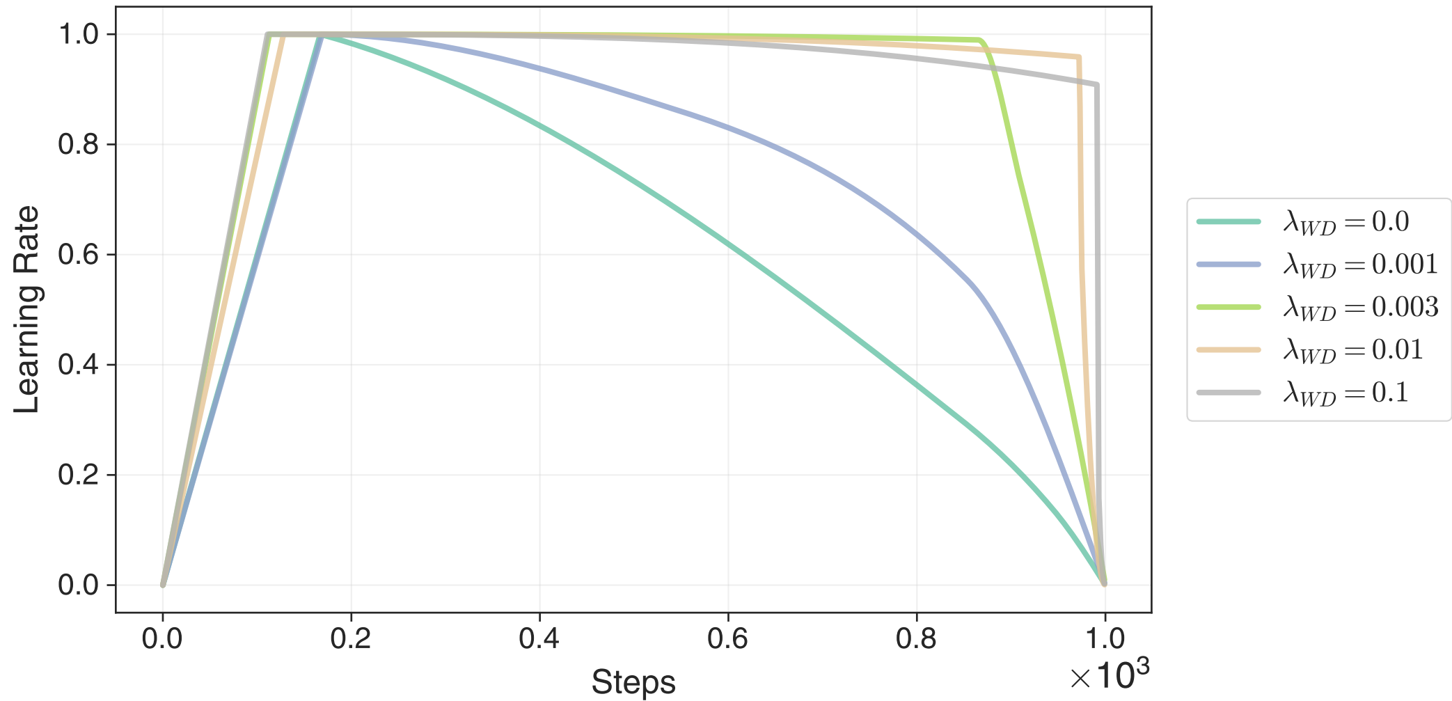
Relative learning rates CIFAR10, varying \lambda_{WD} , TPS schedule
