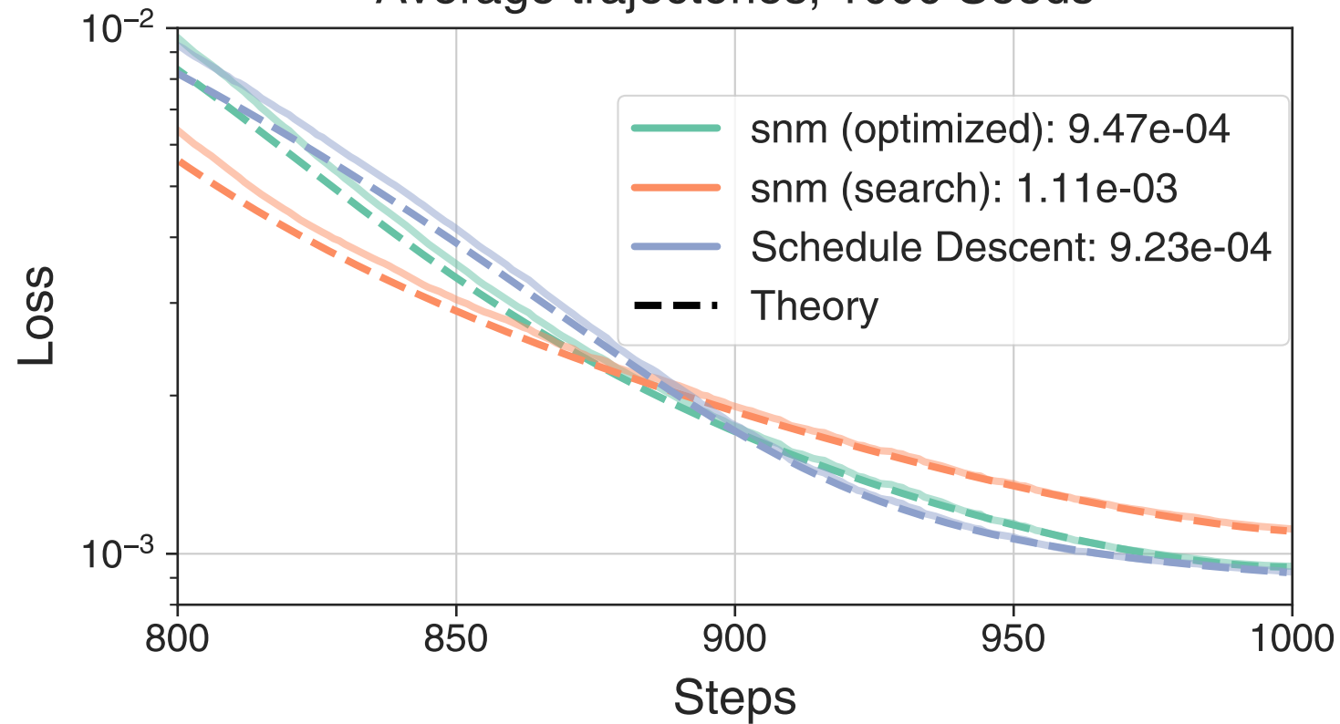
Average trajectories, 1000 Seeds
