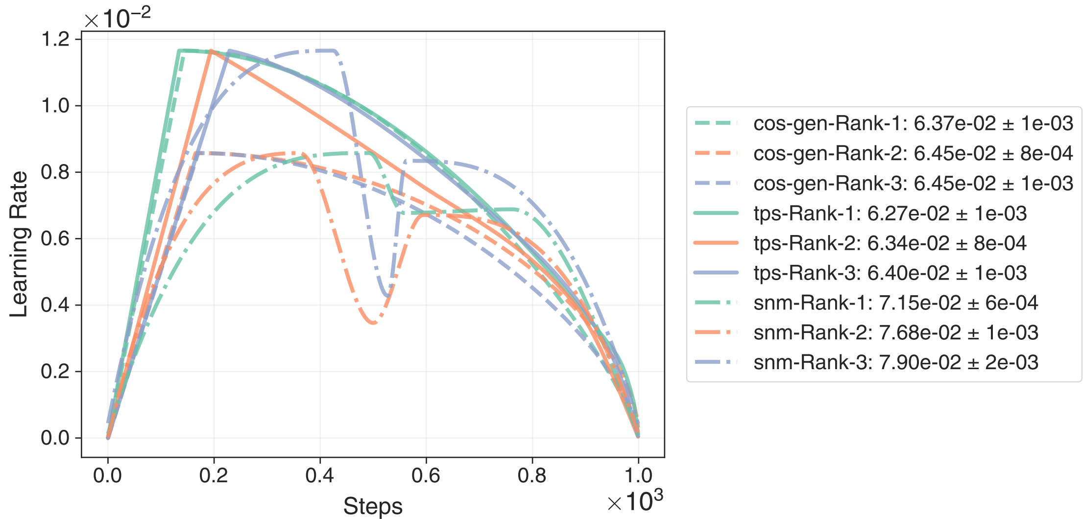
Cifar10 1000steps BS256 Adam Top 3 per family
