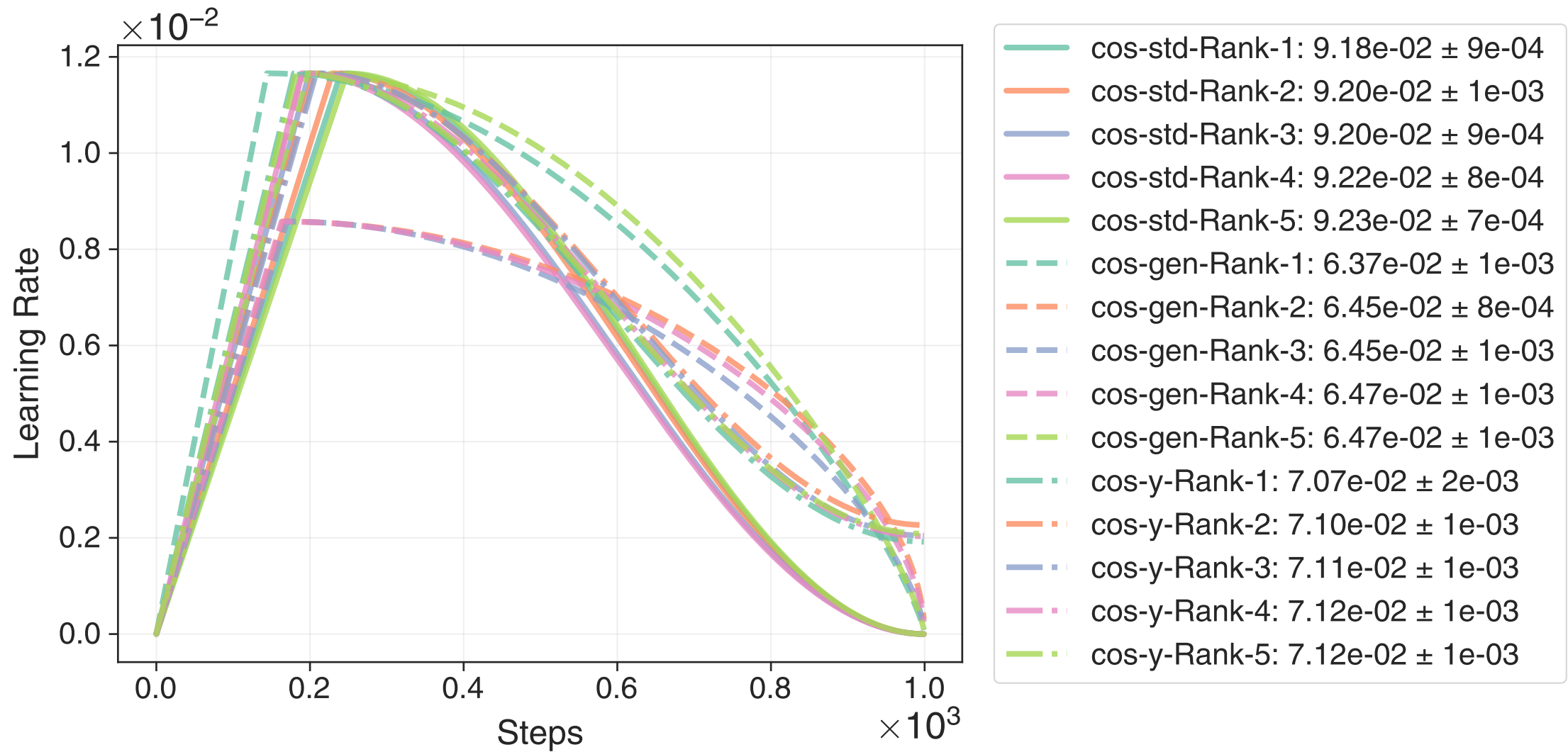
Cifar10 1000steps BS256 Adam Top 5 per family
