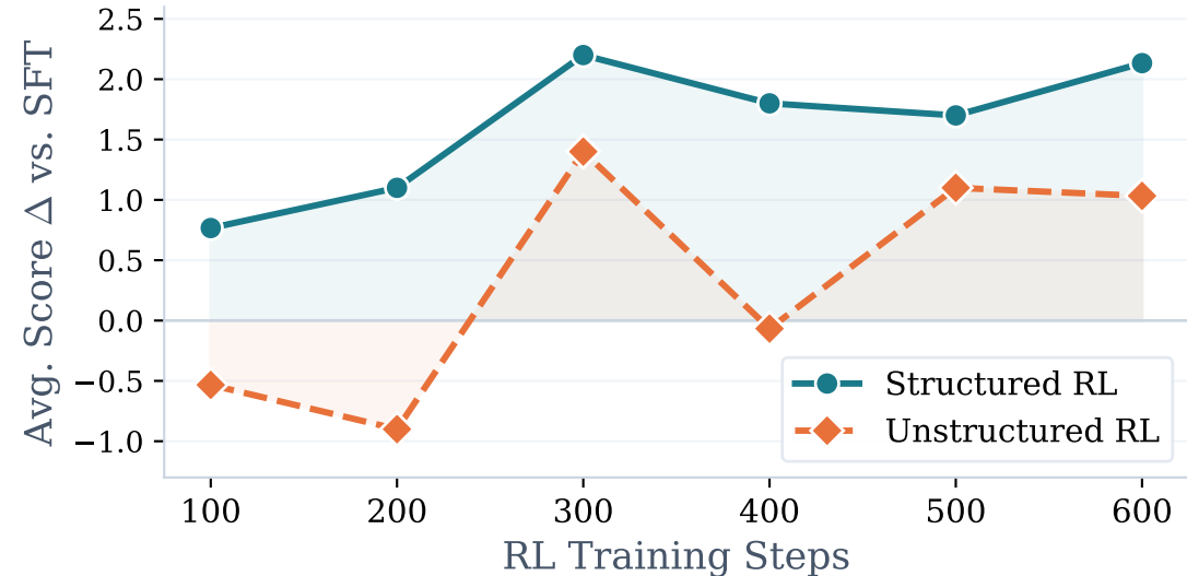
(b) SFT Scaffold Influence on RL Improvements
