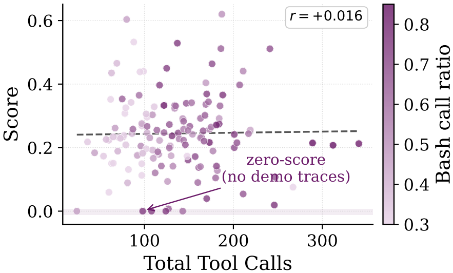
Score vs. Tool Call Count
