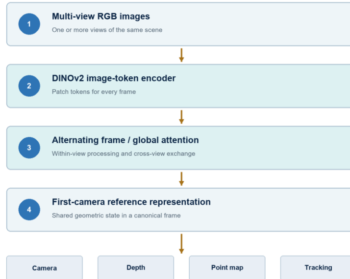
Figure 2. Study-oriented architecture of the maintained VGGT implementation.
