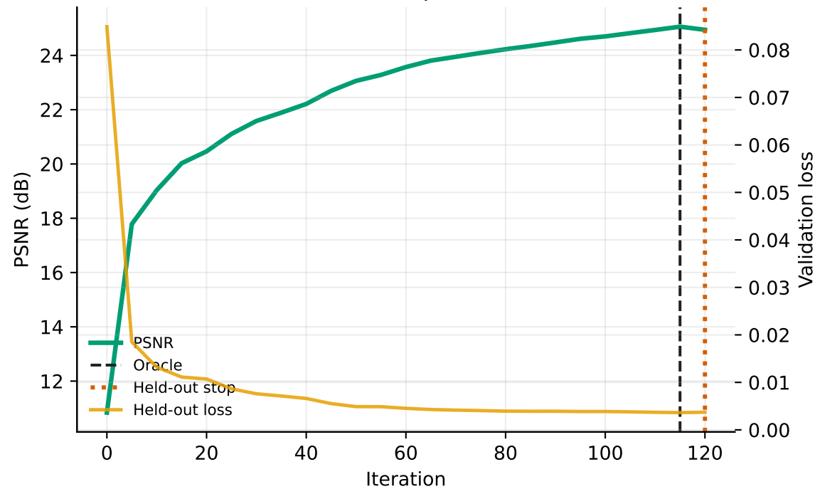
2x SR / pixel
