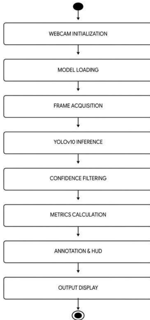
Fig 3.2: Activity Diagram
