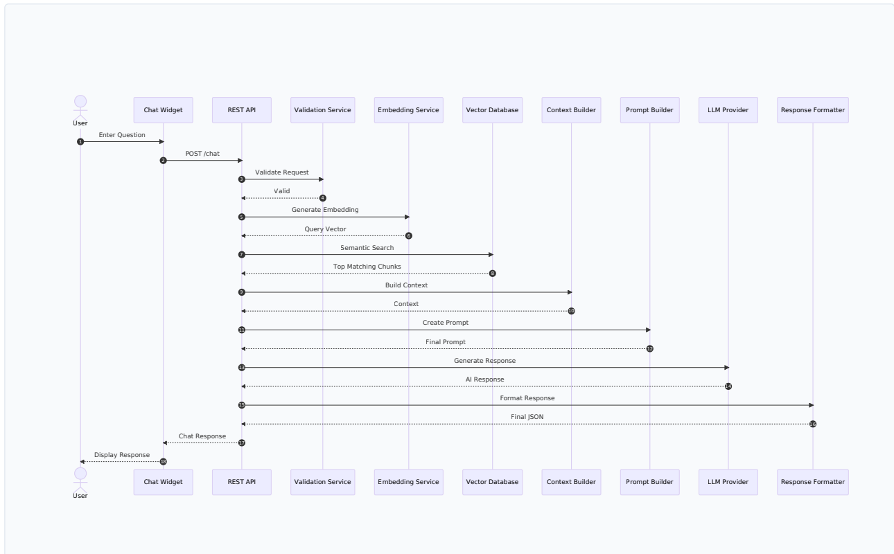
Figure 4.1: Request Processing Sequence
