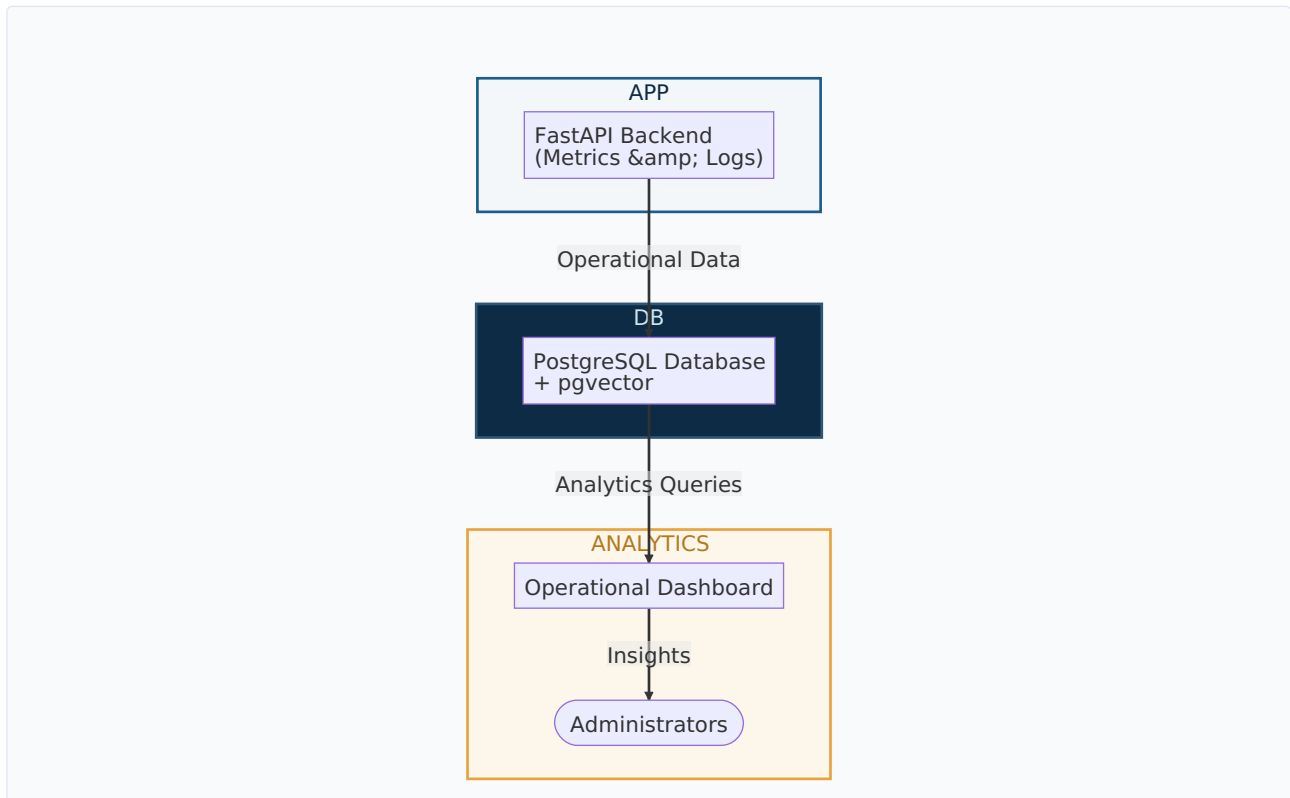
Figure 10.1: Dashboard Architecture Overview
