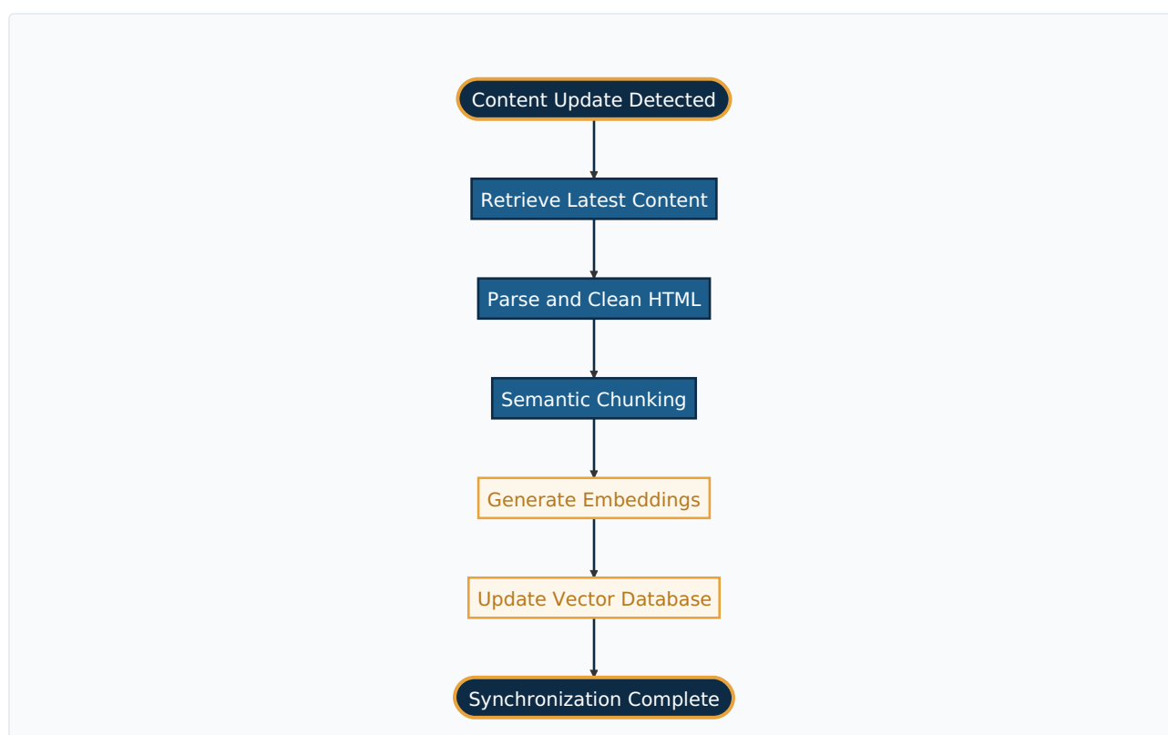
Figure 3.1: Synchronization Workflow
