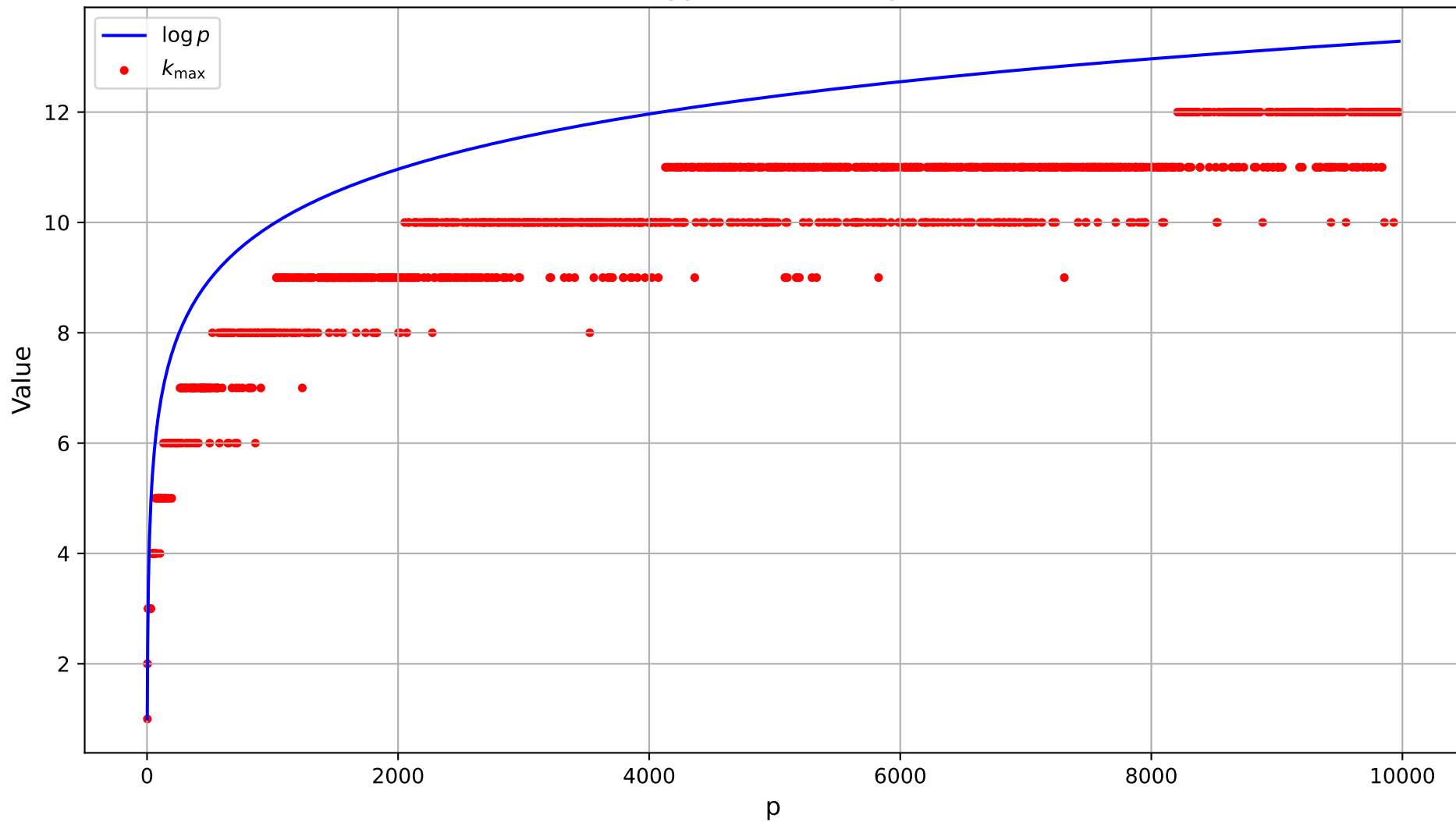
\log p and k_{\max} vs p
