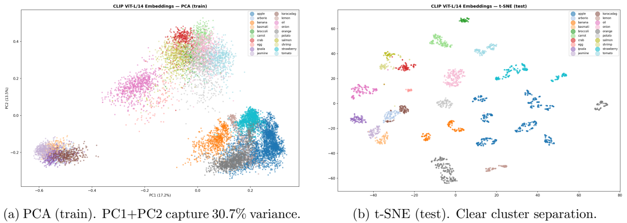
Figure 3: CLIP ViT-L/14 embedding space. All 20 classes form well-separated clusters.
